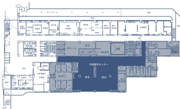
First Floor Plan Scale
